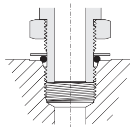
Fig. 3 - Fitting Backed Off for Alignment (1 Turn Maximum)
